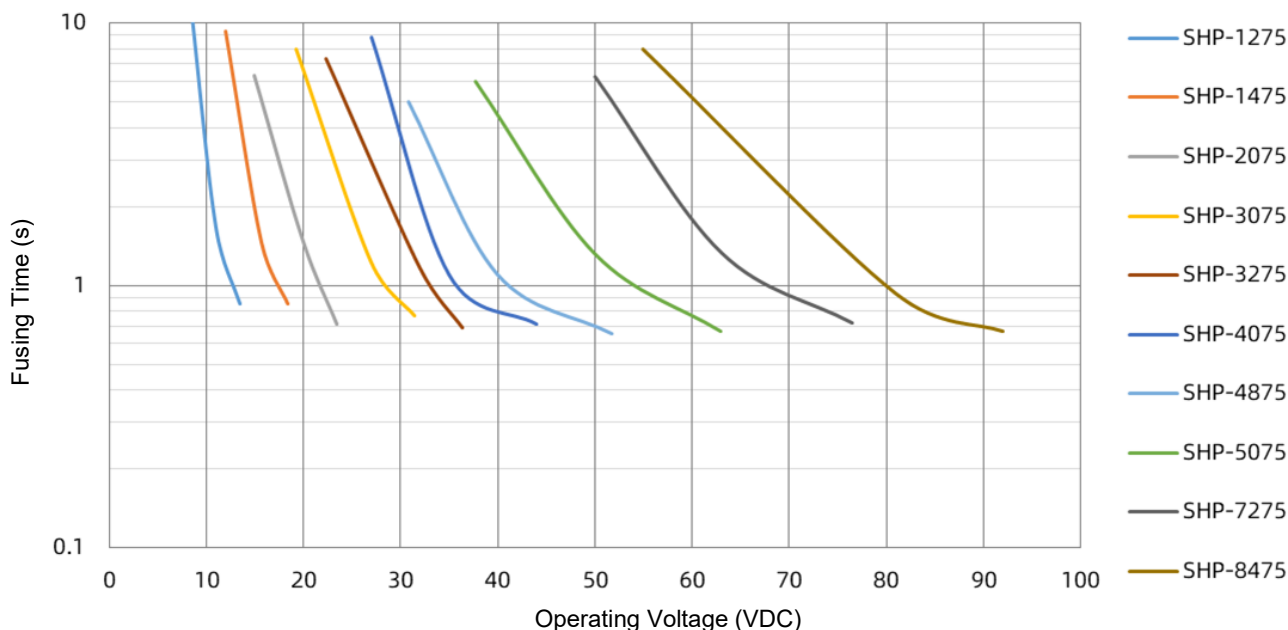
SHP 75 A Controlled Fusing Time Curve
