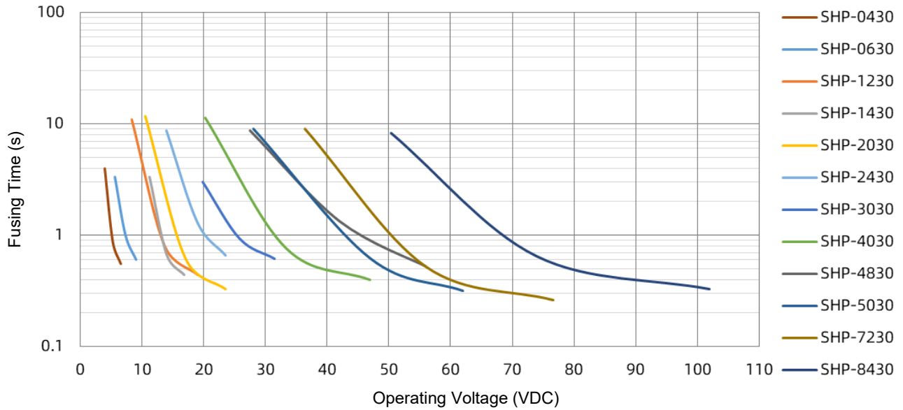
SHP 30 A Controlled Fusing Time Curve
