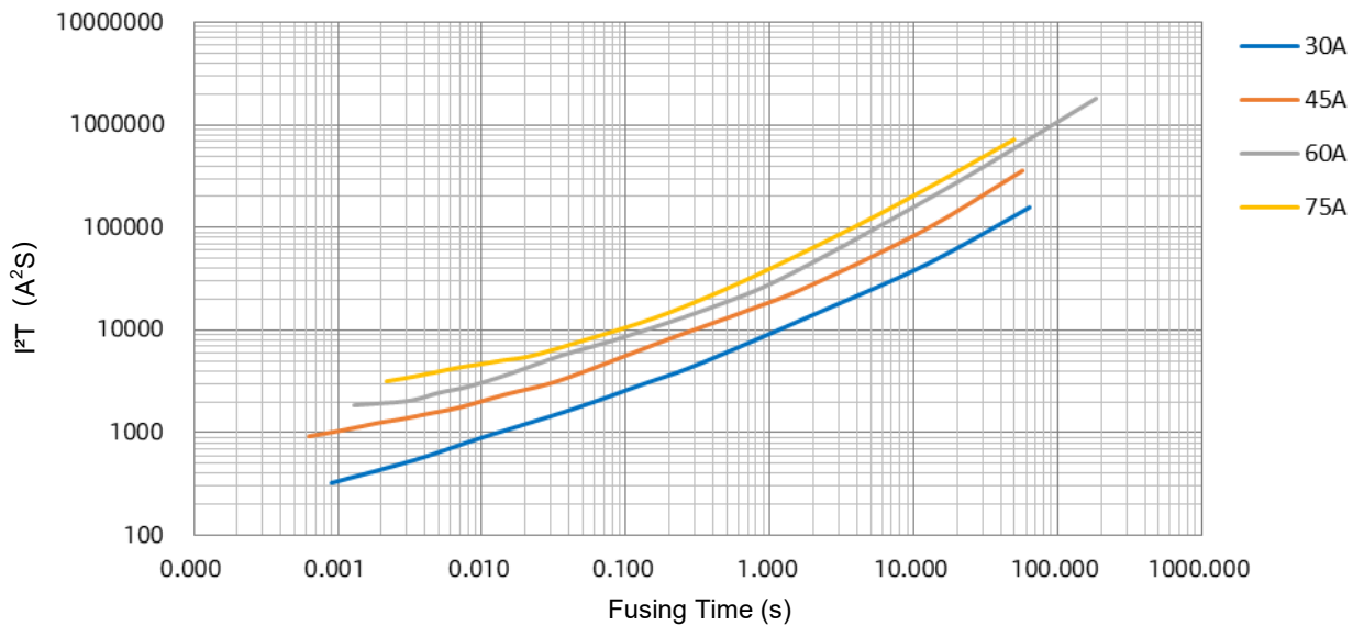
SHP I²t-t Curve
