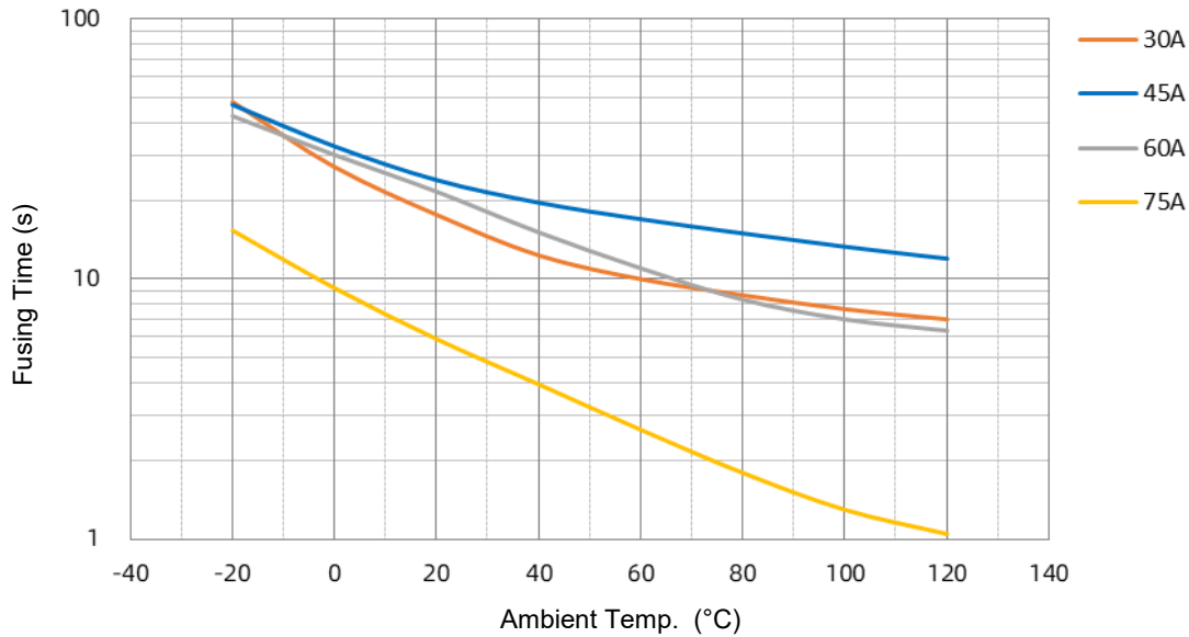
SHP Temp.-Time Curve
