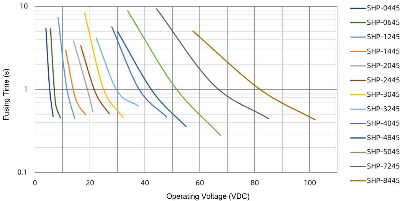
SHP 45 A Controlled Fusing Time Curve
