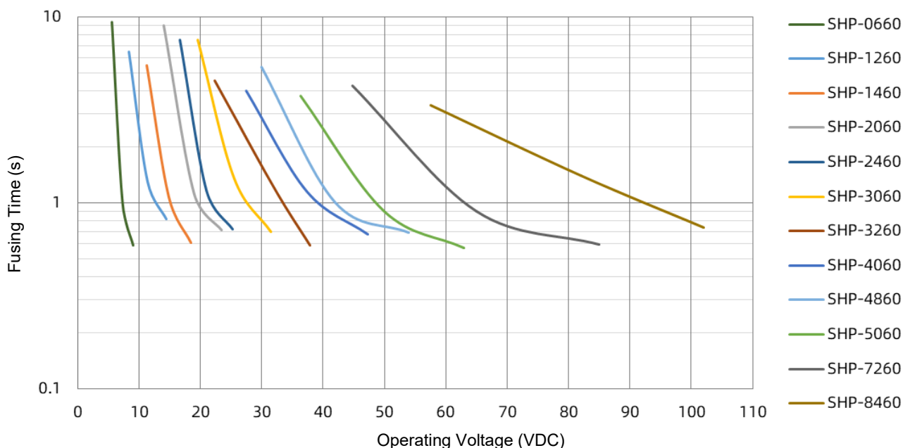
SHP 60 A Controlled Fusing Time Curve
